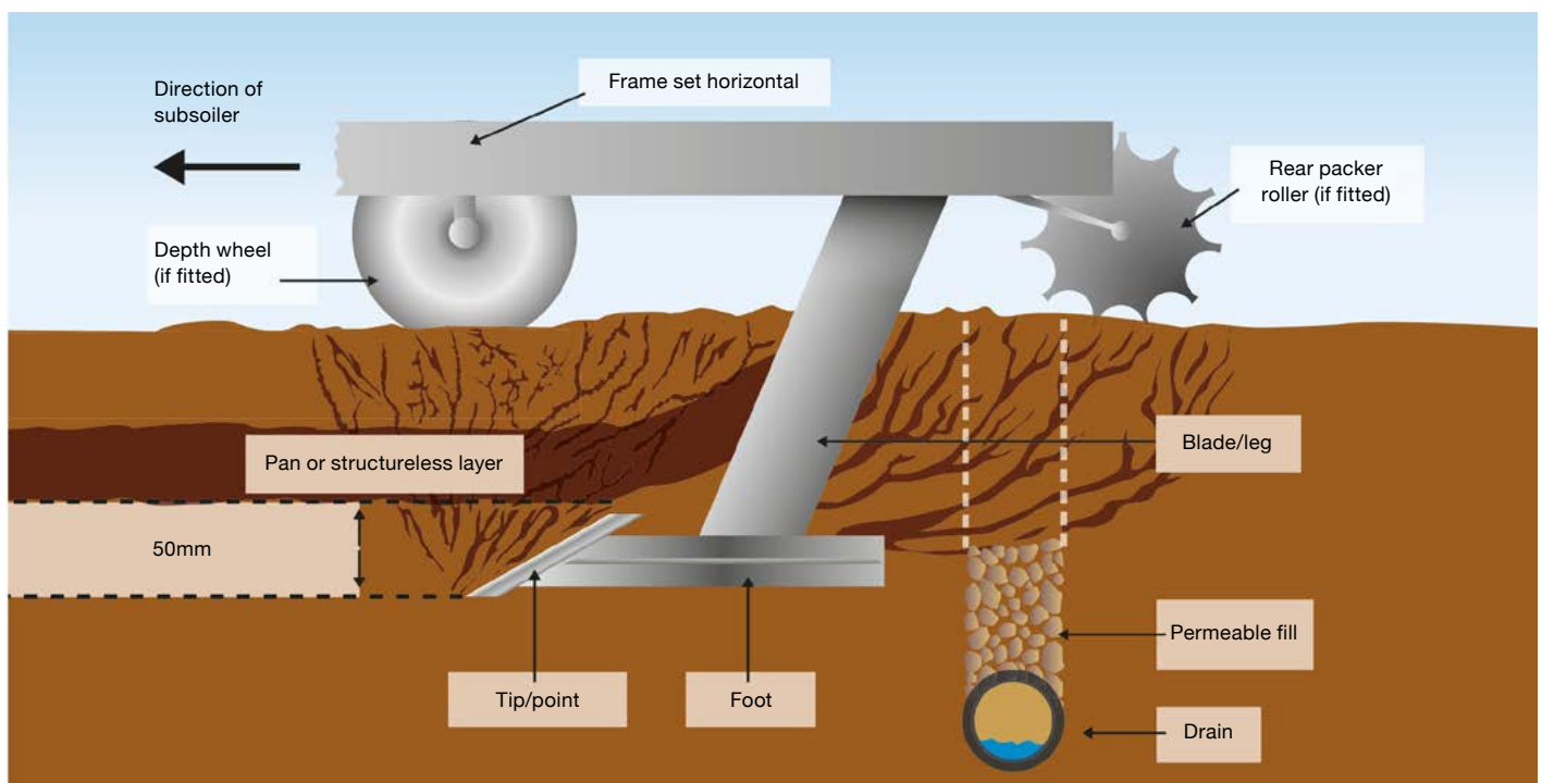
Figure 13. Subsoiler operation
