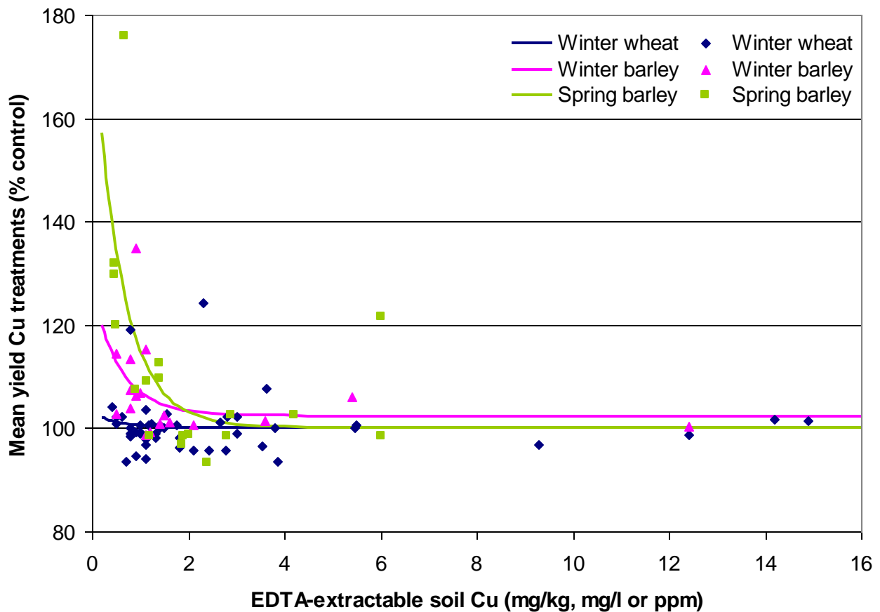
Figure 5. Relationship between EDTA-extractable soil copper levels and cereal yield responses to copper application for winter wheat, winter barley and spring barley ( P < 0.001 ; R^2 = 0.403 ). Mean treated yields are shown as a percentage of untreated control yield, and include foliar treatments, seed treatments, broadcast and soil incorporated treatments.
