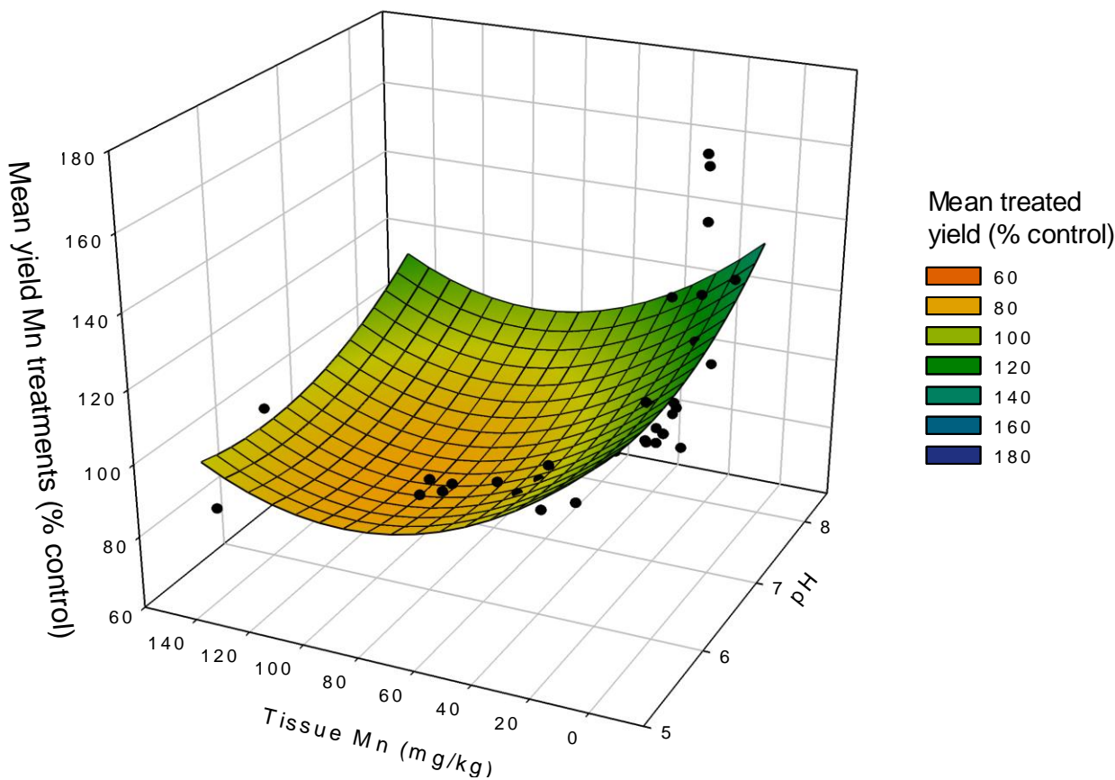
Figure 10. Relationship between yield response to manganese (as % of untreated control yield), soil pH and tissue manganese concentration (mg/kg) for 36 experiments. Paraboloid relationship fitted using Sigma Plot: f = 274.1697 - 51.569x - 0.7103y + 4.3026x^2 + 0.0039y^2 , where x = soil pH, y = tissue Mn and z = yield response. R^2=0.3141 .
