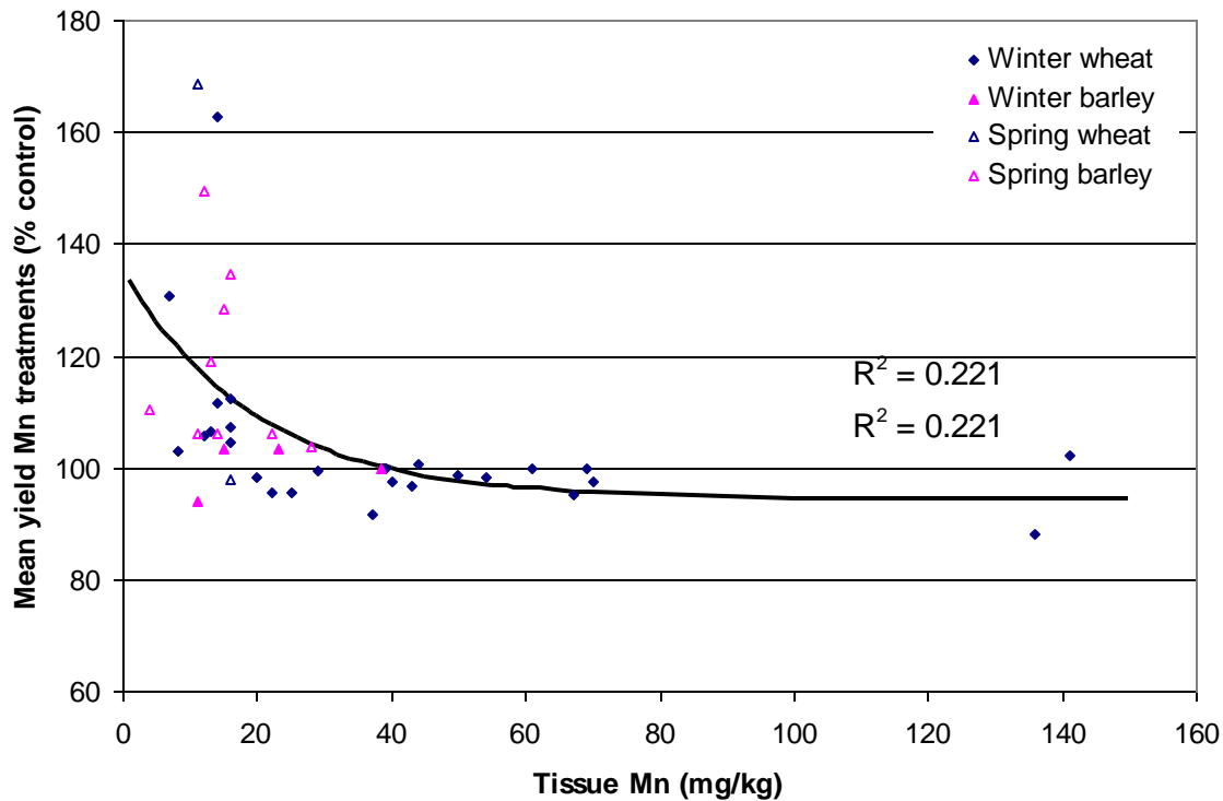
Figure 9. Relationship between tissue manganese levels and cereal yield response to manganese applications (P=0.003). Mean treated yields are shown as a percentage of untreated control yield, and include foliar treatments, seed treatments, broadcast and soil incorporated treatments.
