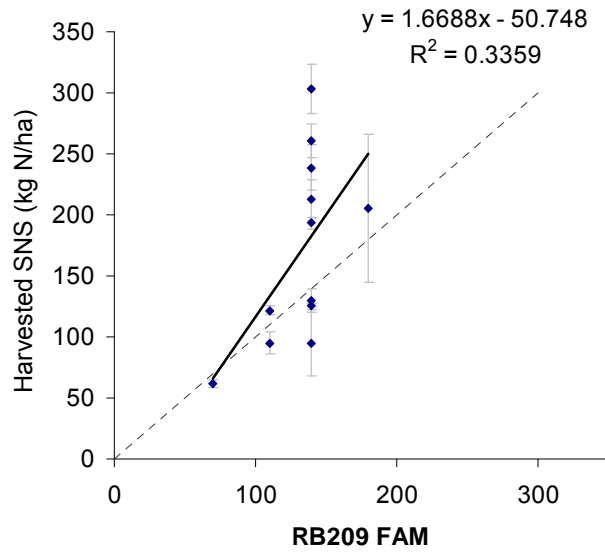
Figure 58. Linear regression for FAM and SMN-based predictions of harvested SNS for cereal crops following vegetable crops in 2008-2010. The dotted line shows y=x .
